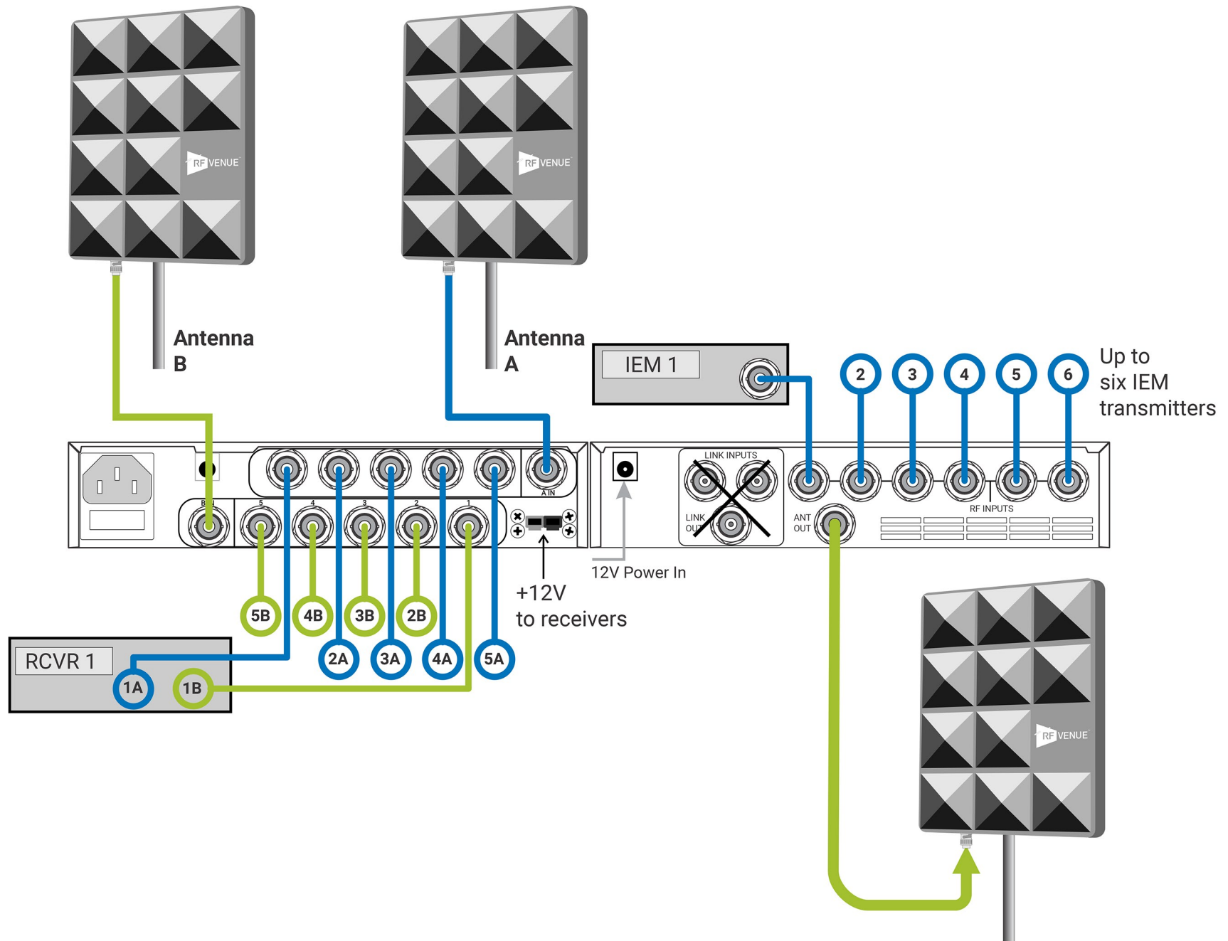
Three CP Stage Antennas and up to 5 mic channels and 6 IEM channels with one DISTR05 HDR and one COMBINE6 HDR
